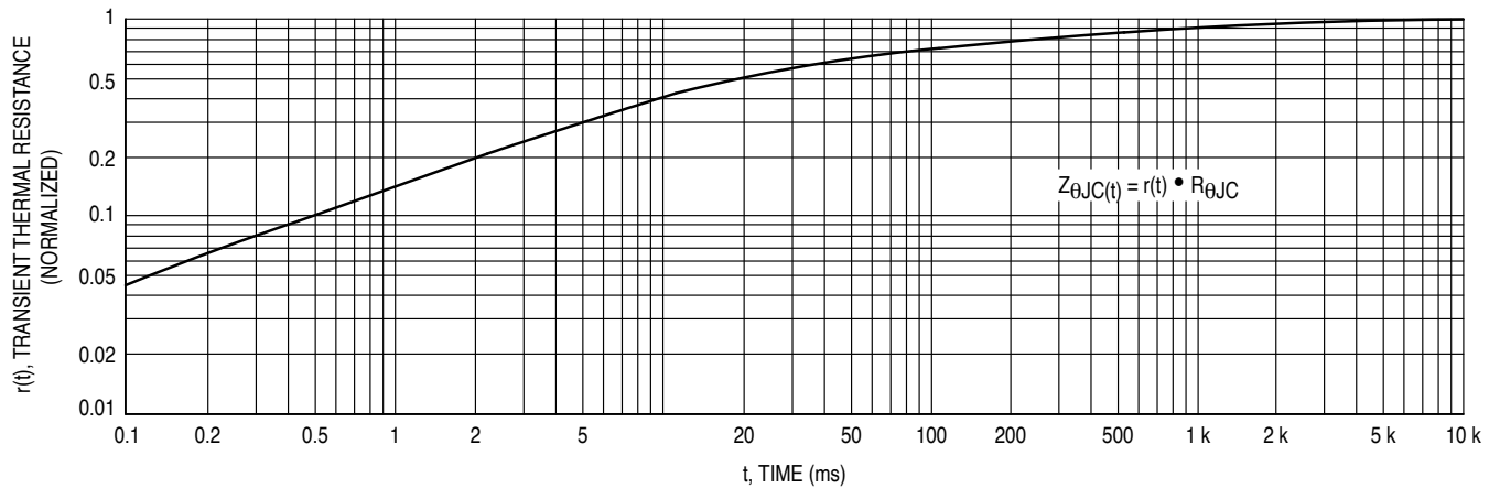
FIGURE 7 – THERMAL RESPONSE
