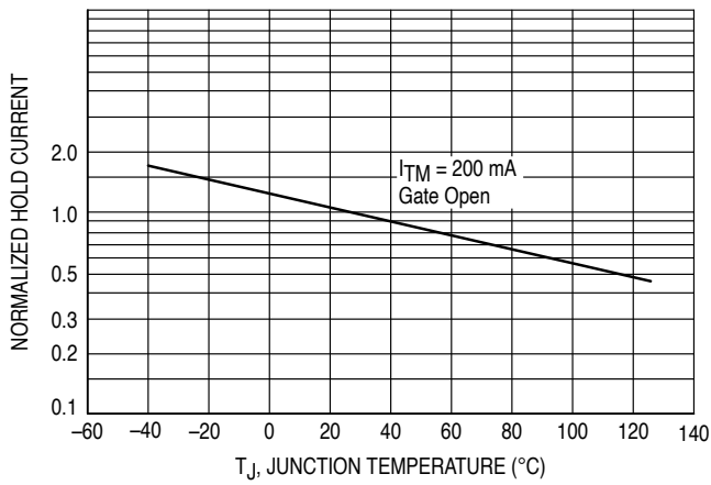
FIGURE 5 – HOLDING CURRENT
