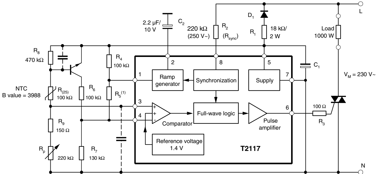
Figure 10-3. Temperature Control 15°C to 35°C with Sensor Monitoring
