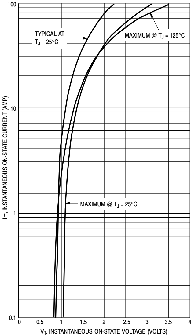
Figure 3. On-State Characteristics
