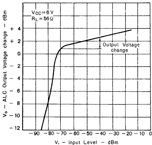
ALC OUTPUT VOLTAGE CHANGE vs. INPUT LEVEL
