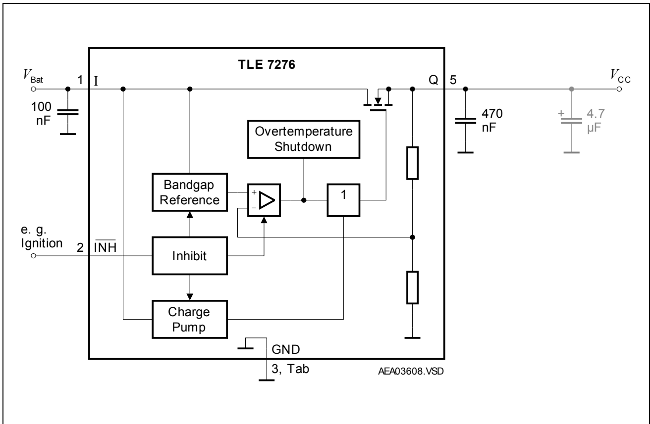
Figure 3 Application Diagram
