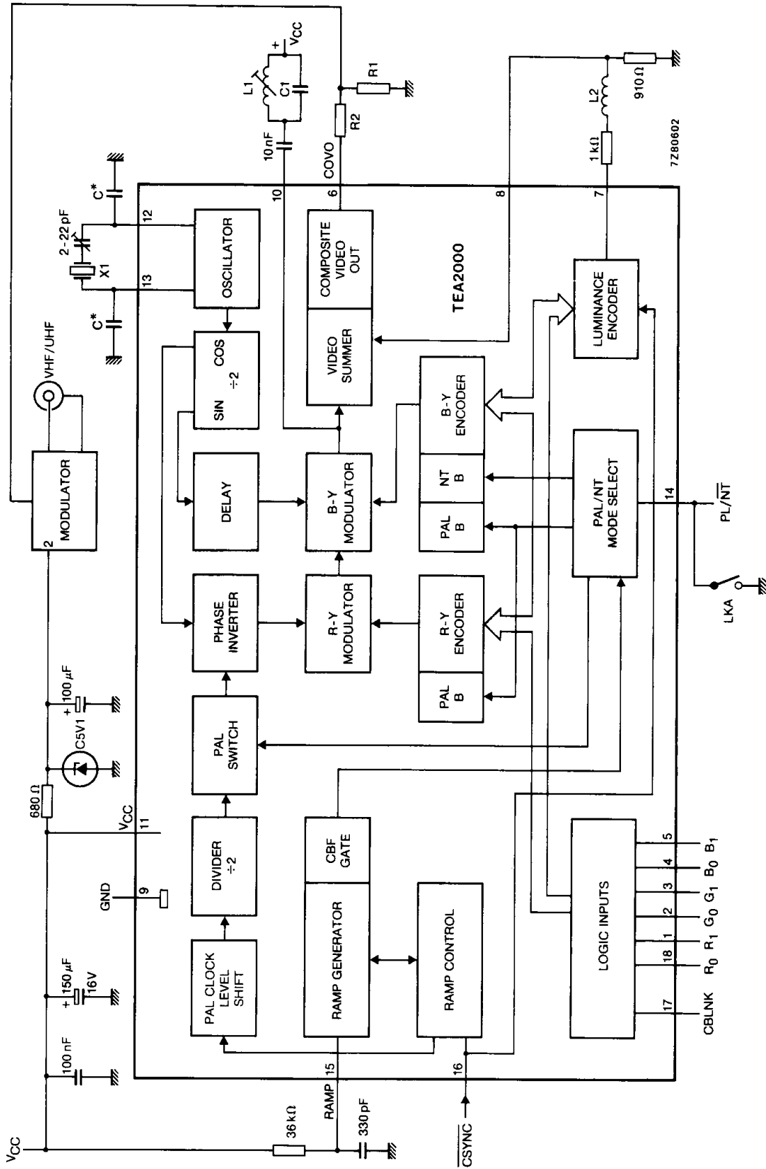
Fig. 2 Internal circuit details and typical external connections.
