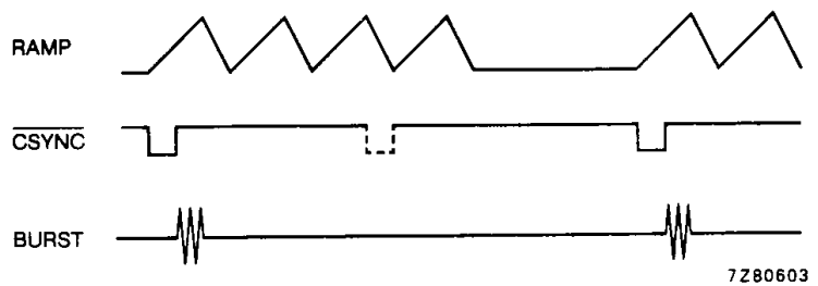
Fig. 3 Ramp timing.
