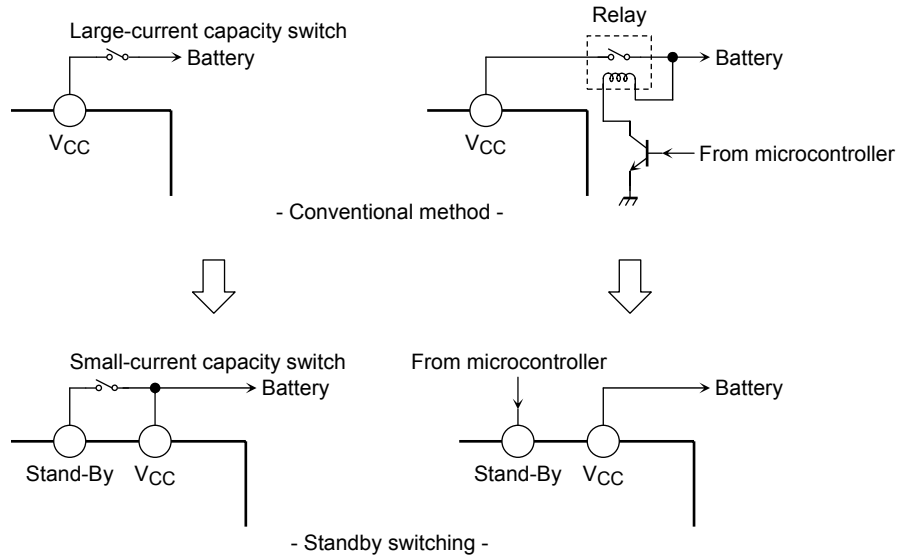
Figure 3 Standby switching
