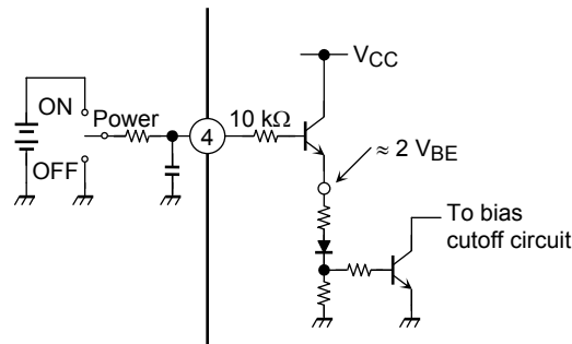
Figure 2 Driving pin 4 high powers up the TB2905HQ
