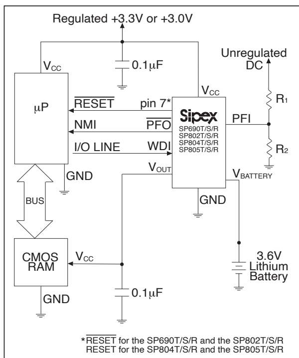
Figure 20. Typical Operating Circuit
