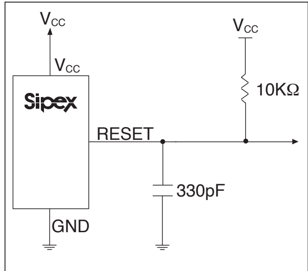
Figure 16B. Circuit for the SP805 RESET Response Time
