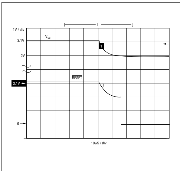
Figure 15A. SP690A \overline{\text{RESET}} Response Time
