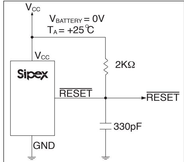
Figure 13B. Circuit for the SP690A/802L \overline{\text{RESET}} Output Voltage vs. Supply Voltage
