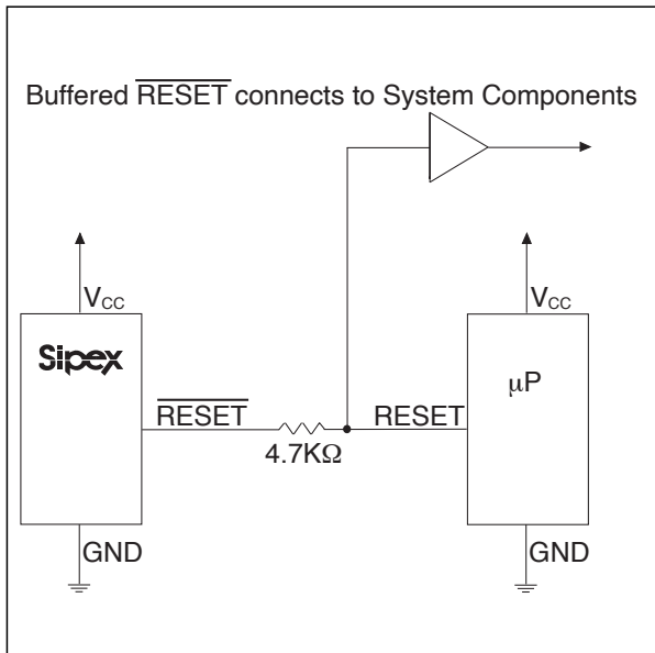
Figure 24. Interfacing to Microprocessors with Bidirectional RESET I/O
