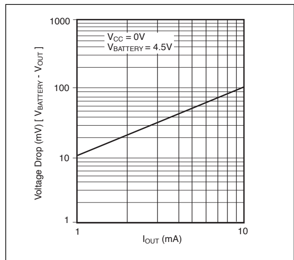
Figure 12. V_{BATTERY} to V_{OUT} Vs. Output Current
