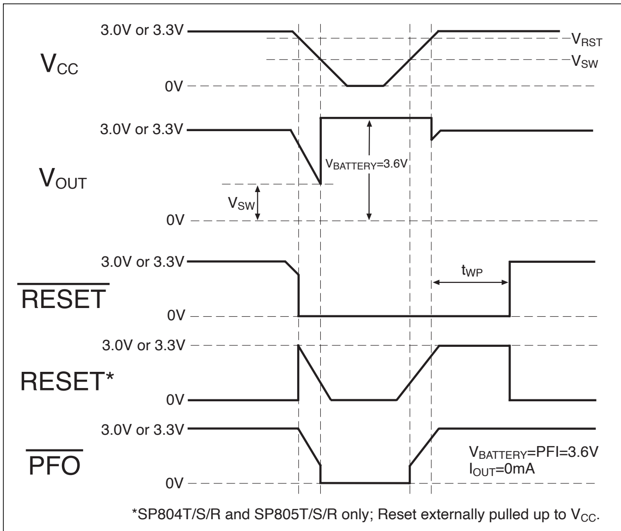
Figure 19. Timing Diagram
