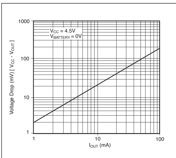
Figure 11. V_{CC} to V_{OUT} Vs. Output Current
