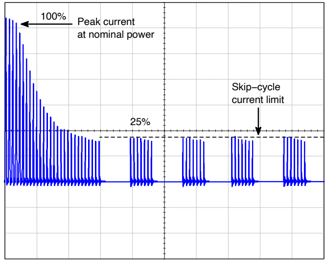
Figure 20. Low Peak Current Skip-Cycle Guarantees Noise-Free Operation
