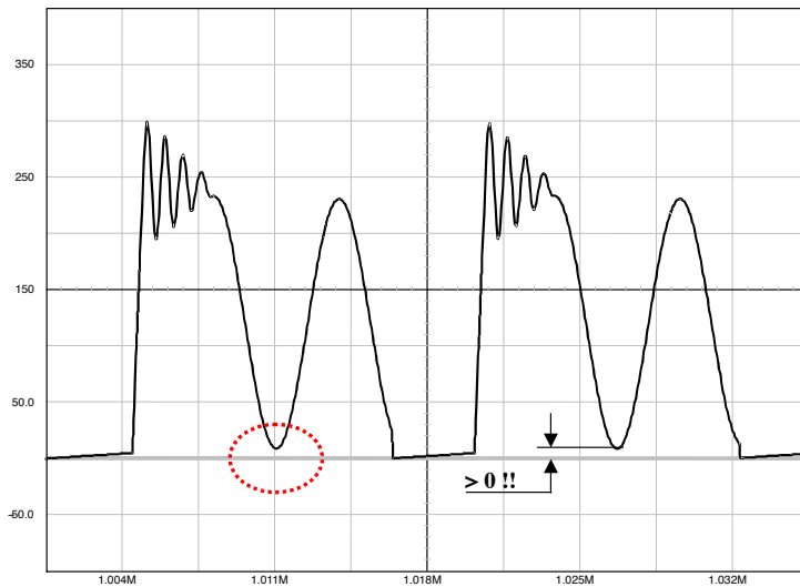
Figure 26. The Drain–Source Wave Shall Always be Positive . . .
