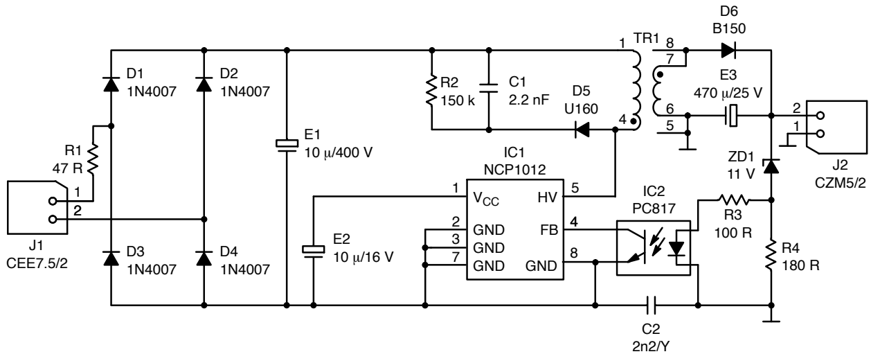
Figure 28. An NCP1012–Based Flyback Converter Delivering 6.5 W
