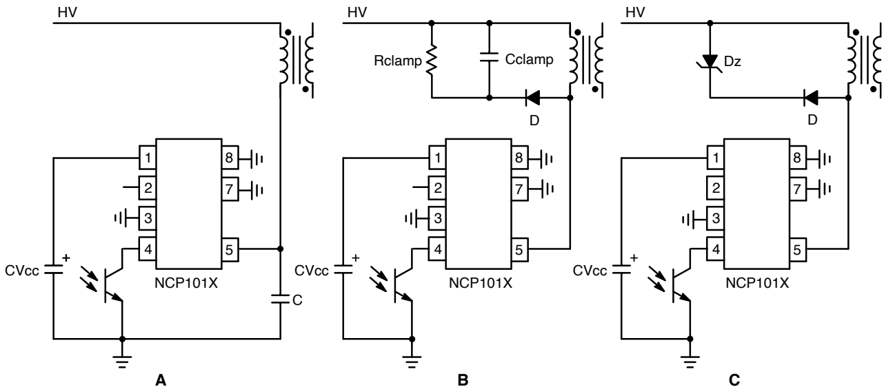
Figure 27. Different Options to Clamp the Leakage Spike
