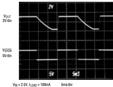
MAX856 START-UP DELAY (5V MODE)
