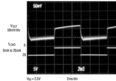
MAX858/MAX859 LOAD-TRANSIENT RESPONSE
