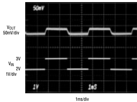
MAX859 LINE-TRANSIENT RESPONSE
