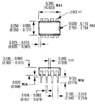
8 Lead Plastic DIP
