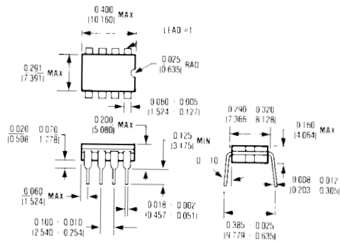
8 Lead Cerdip
