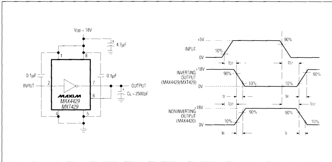
Figure 1. Switching-Time Measurement Circuit
