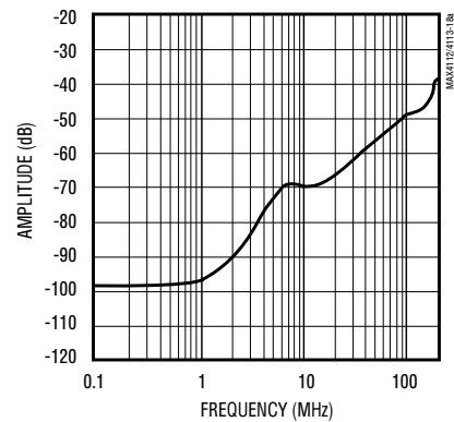
MAX4117-MAX4120 CROSSTALK vs. FREQUENCY
