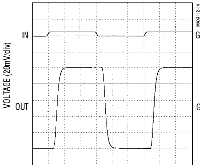
MAX4113/MAX4118/MAX4120 SMALL-SIGNAL PULSE RESPONSE ( A_{VCL} = +20 )
