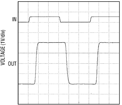
MAX4113/MAX4118/MAX4120 LARGE-SIGNAL PULSE RESPONSE ( A_{VCL} = +8 )
