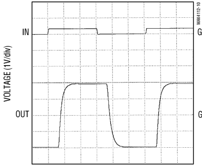
MAX4112/MAX4117/MAX4119 LARGE-SIGNAL PULSE RESPONSE ( A_{VCL} = +10 )
