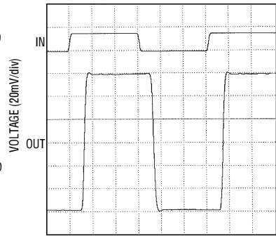
MAX4113/MAX4118/MAX4120 SMALL-SIGNAL PULSE RESPONSE ( A_{VCL} = +8 )
