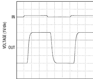
MAX4113/MAX4118/MAX4120 LARGE-SIGNAL PULSE RESPONSE ( A_{VCL} = +20 )
