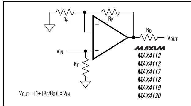
Figure 2b. Noninverting Gain Configuration
