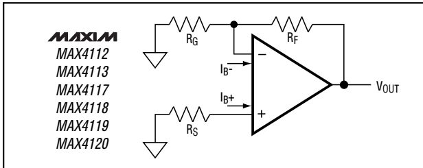
Figure 3. Output Offset Voltage
