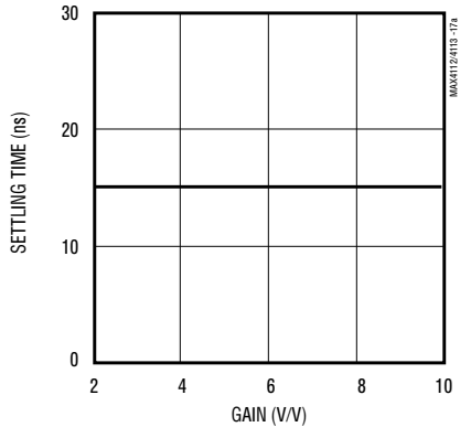
MAX4112/MAX4117/MAX4119 SETTLING TIME vs. GAIN
