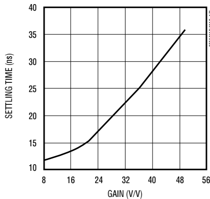
MAX4113/MAX4118/MAX4120 SETTLING TIME vs. GAIN
