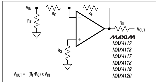
Figure 2a. Inverting Gain Configuration
