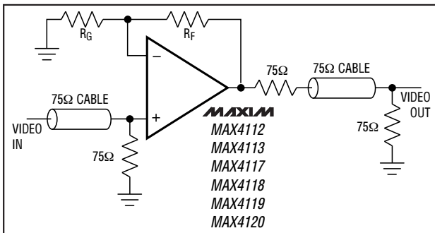
Figure 4. Video Line Driver
