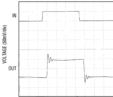
MAX4112/MAX4117/MAX4119 SMALL-SIGNAL PULSE RESPONSE ( A_{VCL} = +2 , C_L = 10pF )
