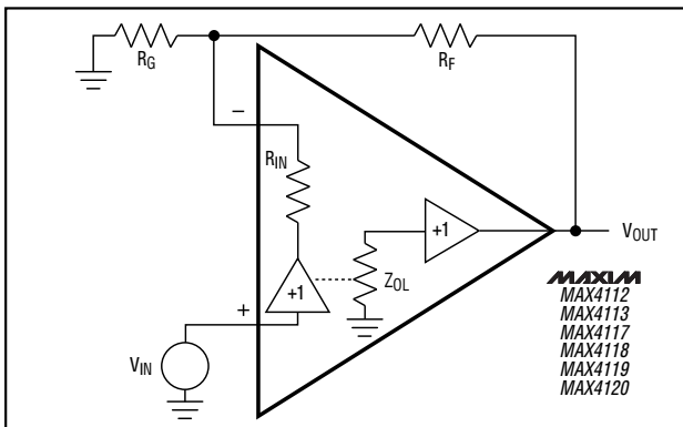
Figure 1. Current Feedback Amplifier
