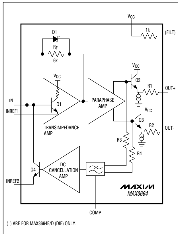
Figure 1. Functional Diagram
