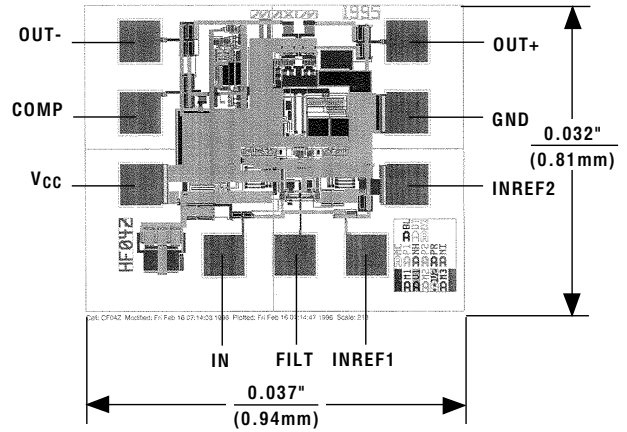
Chip Topography
