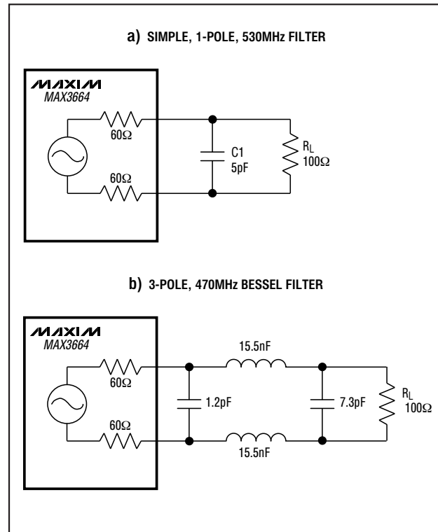
Figure 3. Filter Design Examples
