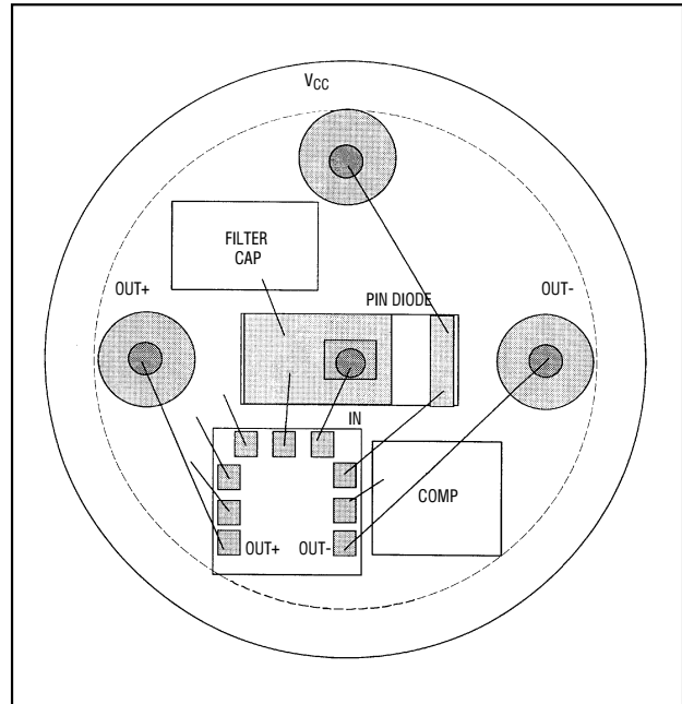
Figure 4. Suggested Layout for TO-46 Header
