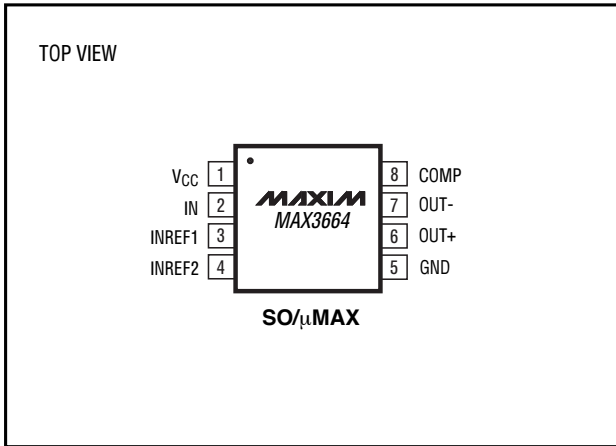
Pin Configuration
