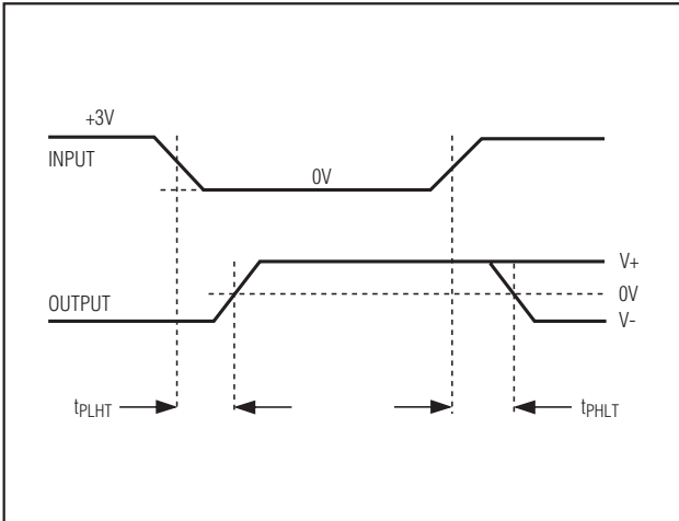
Figure 1. Transmitter Propagation-Delay Timing
