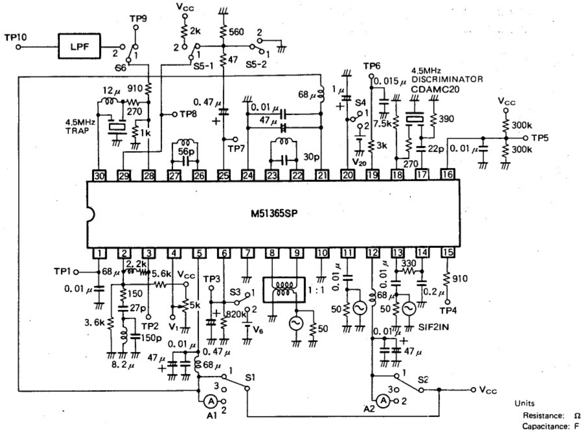
TEST CIRCUIT 2
