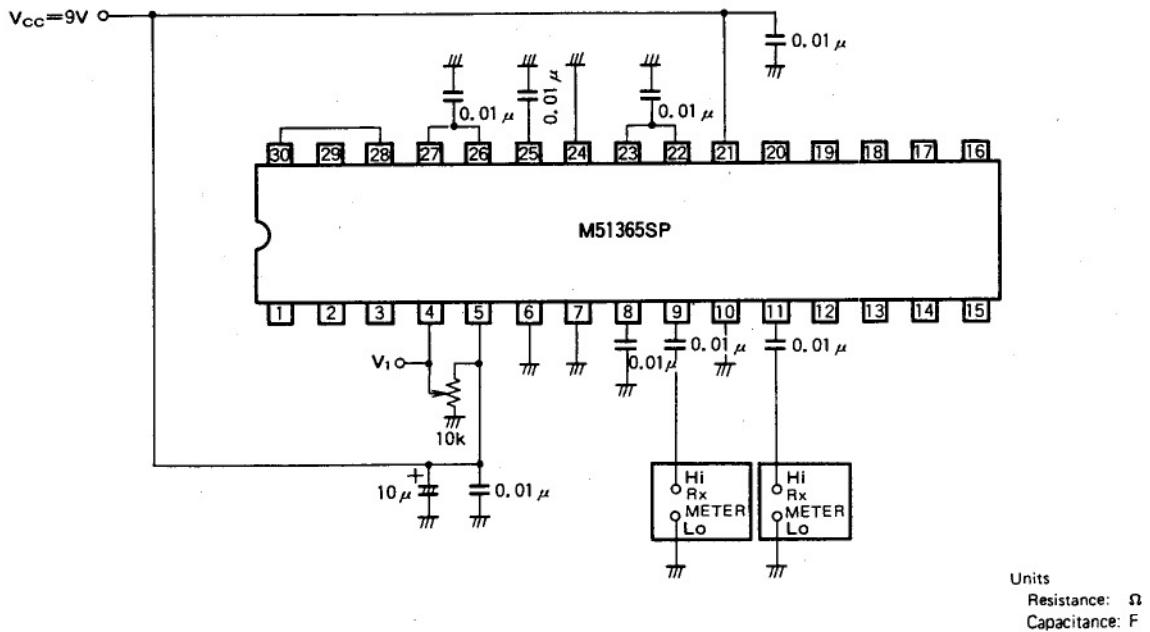
TEST CIRCUIT 2
