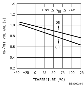
ON/OFF Threshold
