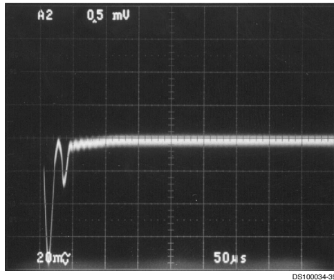
Transient Response with Output Capacitor Halved
