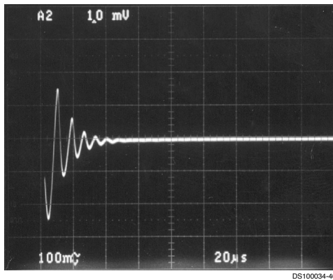
Transient Response with Only 4.7 \mu\text{F} Output Cap
