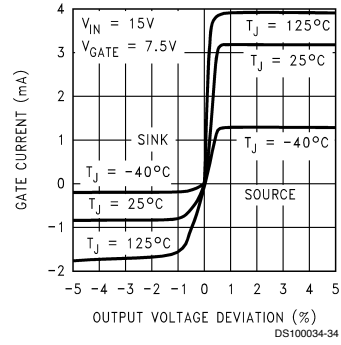
Gate Current
