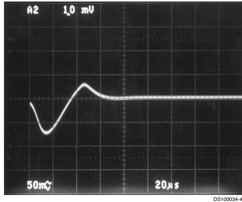
Transient Response for 0–6A Load Step
