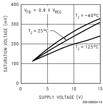
Gate-Ground Saturation
