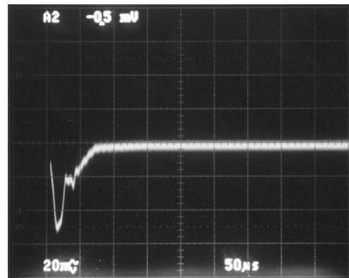
Transient Response for 0–0.5A Load Step
