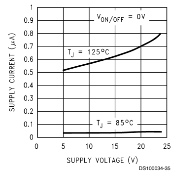
Leakage Current
