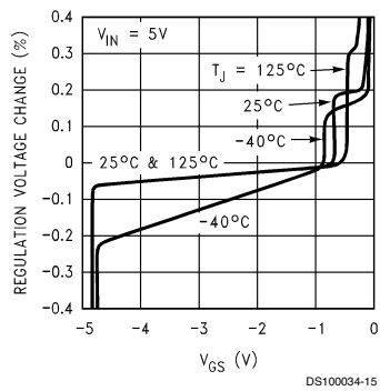
Load Regulation
