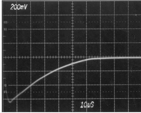
Transient Response for 0–0.5A Load Step
