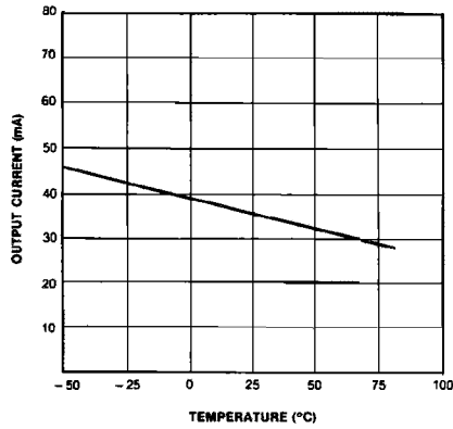
Fig. 9 CURRENT LIMITING
