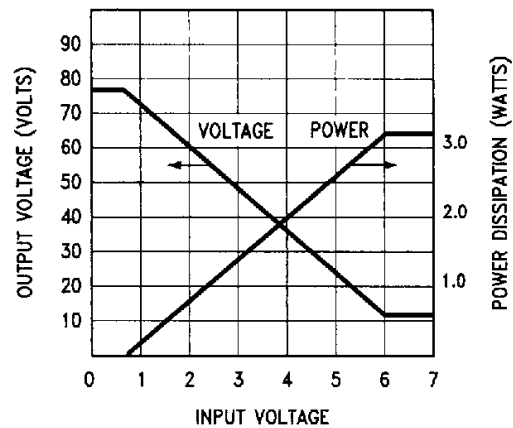
FIGURE 3. LM2416 DC Characteristics
