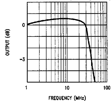
LM2416 Frequency Response
