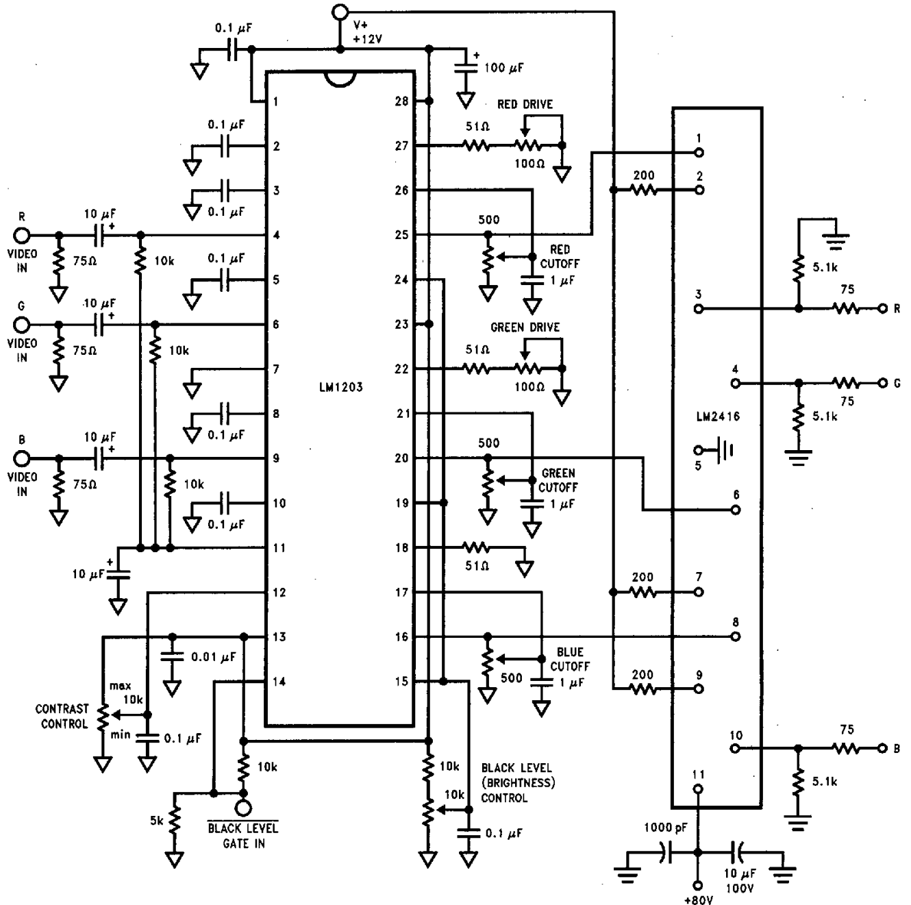
FIGURE 4. Typical Application LM1203-LM2416 Application
