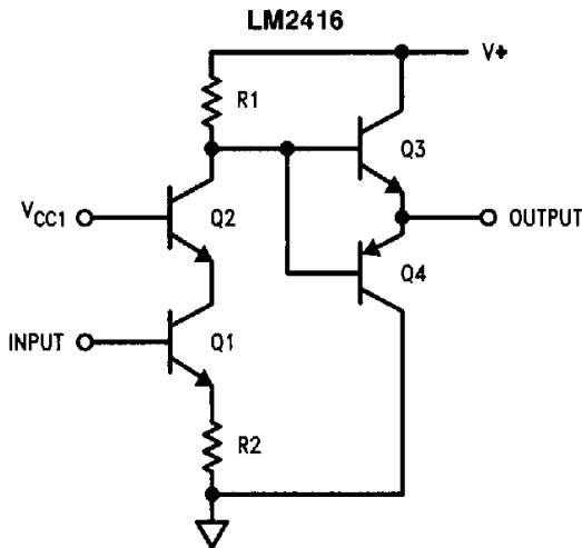
FIGURE 2. LM2416 CRT Driver (One Section)
