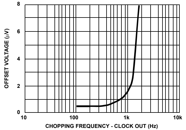
FIGURE 14. INPUT OFFSET VOLTAGE vs CHOPPING FREQUENCY
