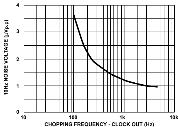
FIGURE 12. 10Hz NOISE VOLTAGE vs CHOPPING FREQUENCY
