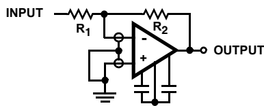
FIGURE 1A. INVERTING AMPLIFIER
