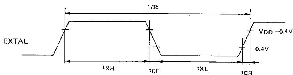
Fig. 1 Clock timing
