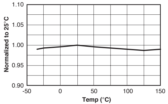
Sync. Threshold in Extended QR(L)
