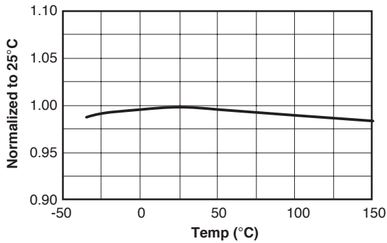
Sync. Threshold in Extended QR(H)
