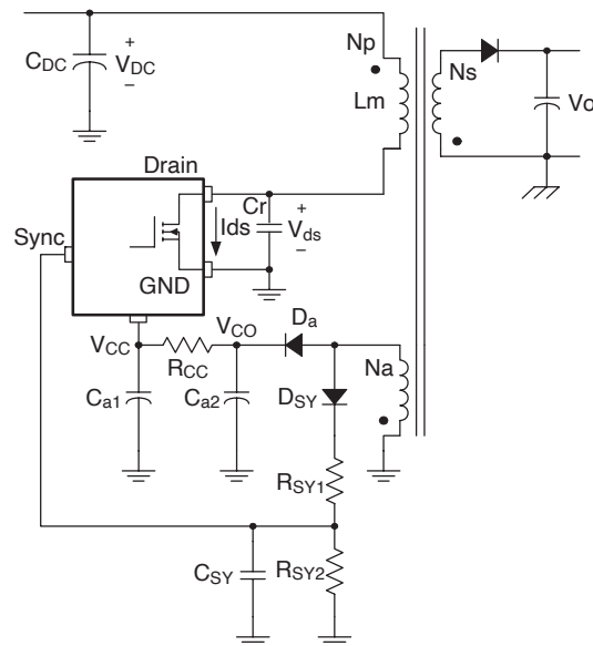
Figure 6. Synchronization Circuit
