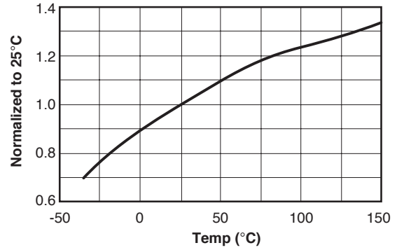
Burst Mode Enable Feedback Voltage
