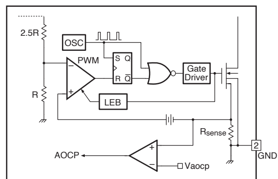
Figure 14. AOCP Block
