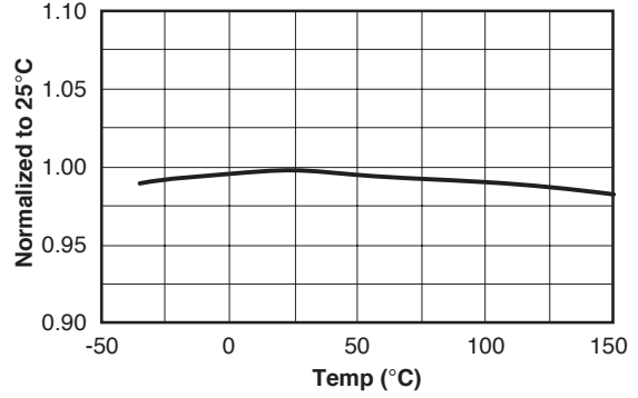
Sync. Threshold in Normal QR(L)
