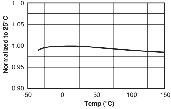
Sync. Threshold in Normal QR(H)
