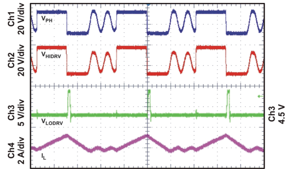
DISCONTINUOUS CONDUCTION MODE (DCM) SWITCHING WAVEFORMS
