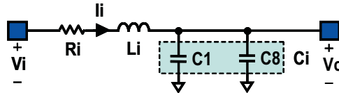
Figure 29. Simplified Equivalent Circuit During Adapter Insertion
