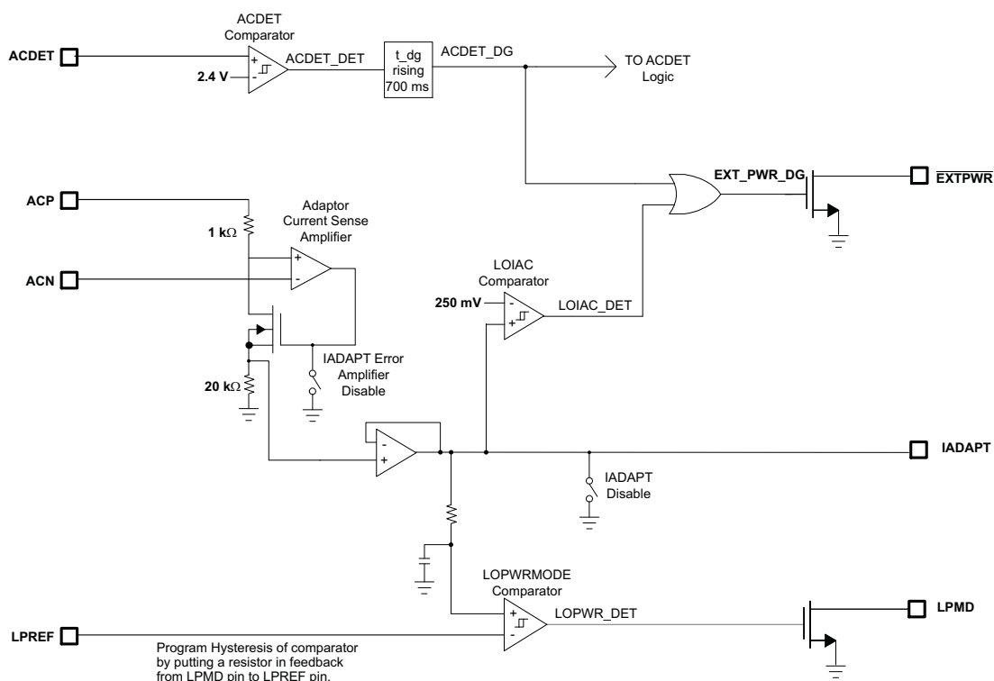
Figure 28. EXTPWR, LPREF and LPMD Logic
