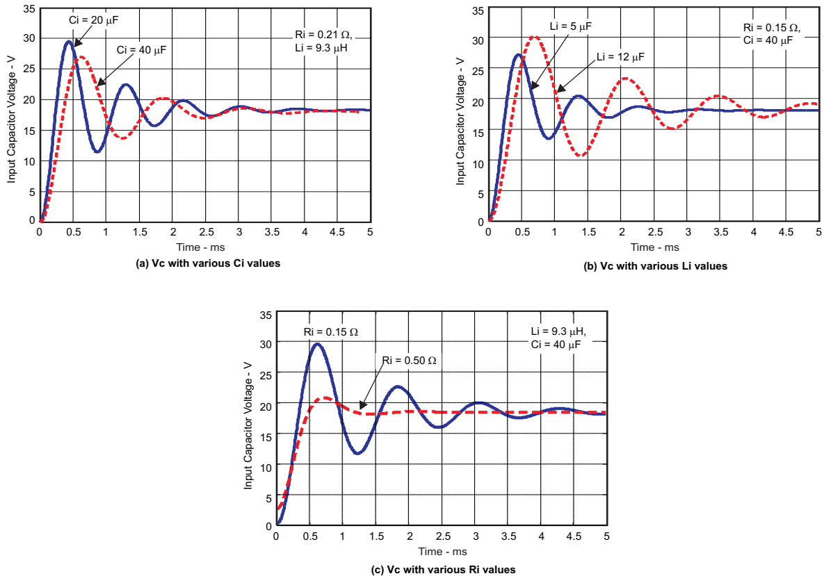
Figure 30. Parametric Study Of The Input Voltage
