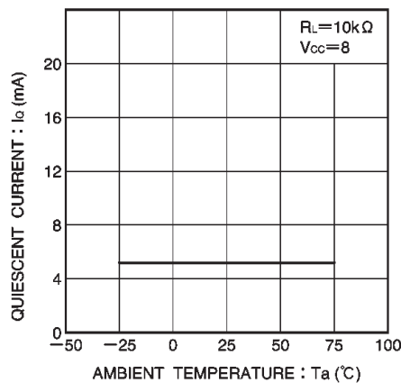
Fig. 6 Quiescent current vs. ambient temperature
