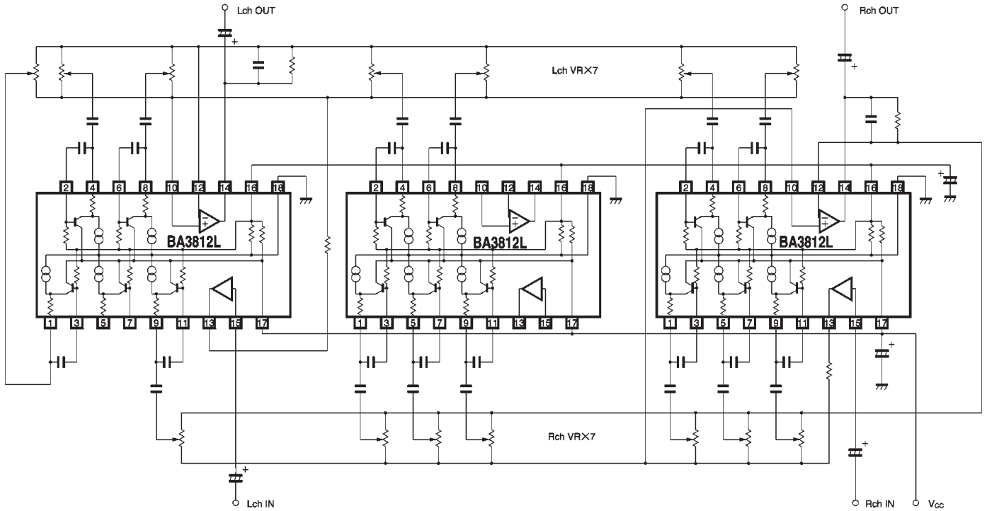
Fig. 3 7-point stereo graphic equalizer circuit
