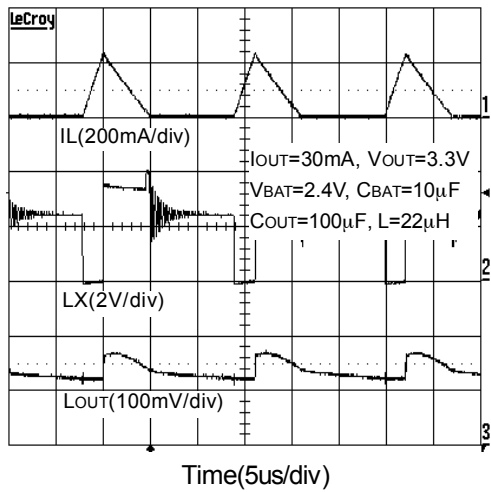
Light Load Operating Waveforms
