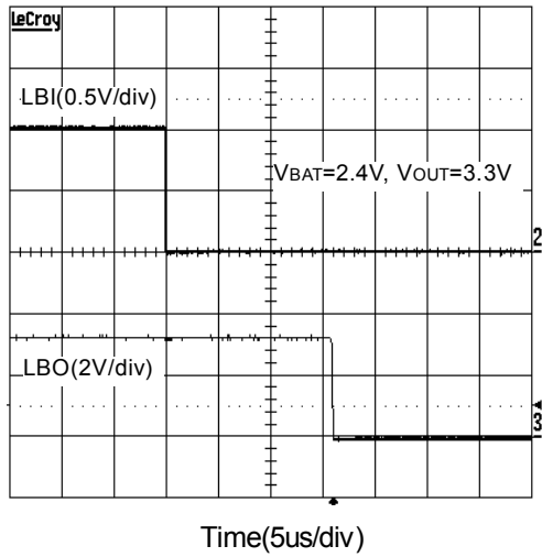
LBO Falling Delay Time
