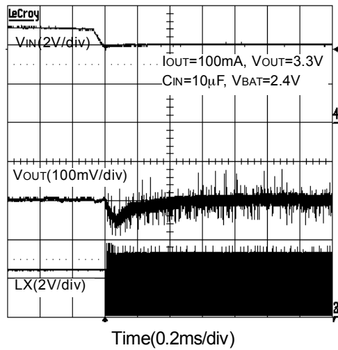
LDO to PWM
