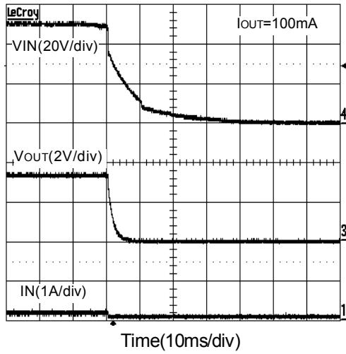
LDO Power Down
