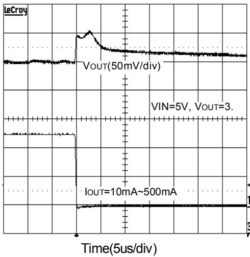
LDO Load Transient Response
