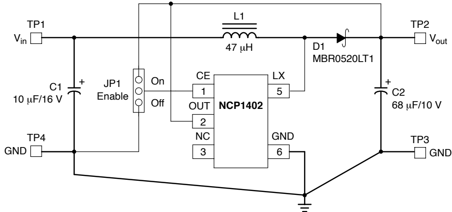
Figure 62. NCP1402 Evaluation Board Schematic Diagram
