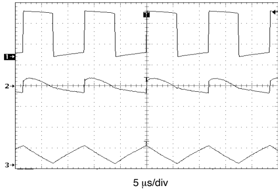
V_{OUT} = 1.9\text{ V} , V_{in} = 1.2\text{ V} , I_O = 30\text{ mA} , L = 47\text{ }\mu\text{H} , C_{OUT} = 68\text{ }\mu\text{F} 1. V_{LX} , 1.0 V/div 2. V_{OUT} , 20 mV/div, AC coupled 3. I_L , 100 mA/div
