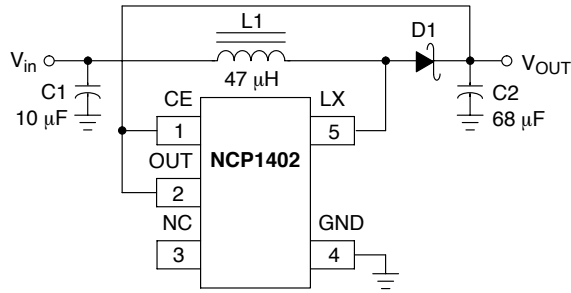
Figure 59. Typical Application Circuit
