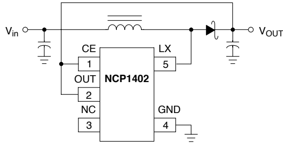
Figure 1. Typical Step-Up Converter Application
