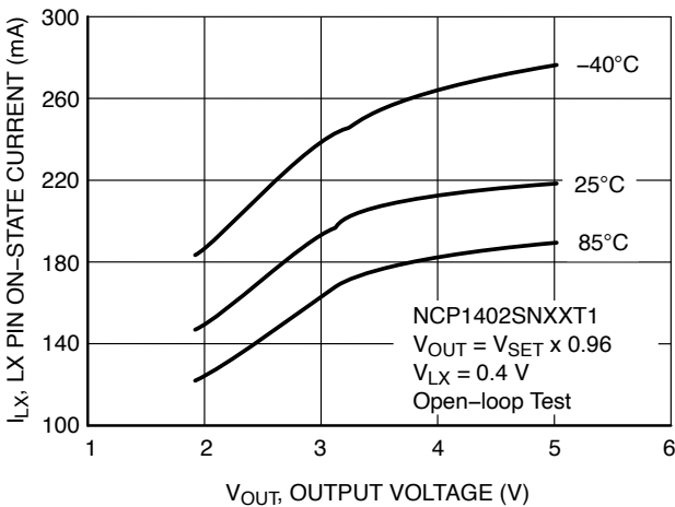
Figure 55. NCP1402SNXXT1 Pin On-state Current vs. Output Voltage
