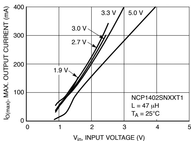
Figure 58. NCP1402SNXXT1 Maximum Output Current vs. Input Voltage
