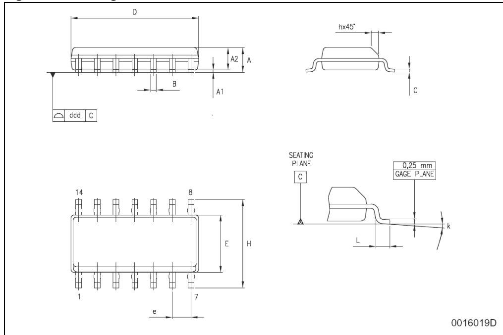
Figure 56. Package dimensions
