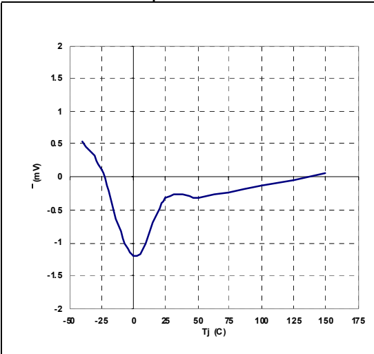
Figure 22. V MULTpk - V VFF dropout vs T J
