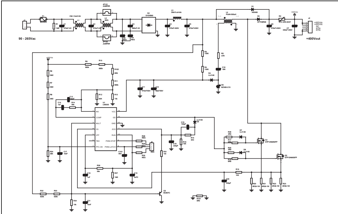
Figure 54. EVL6563S-400W FOT PFC demonstration board: electrical schematic
