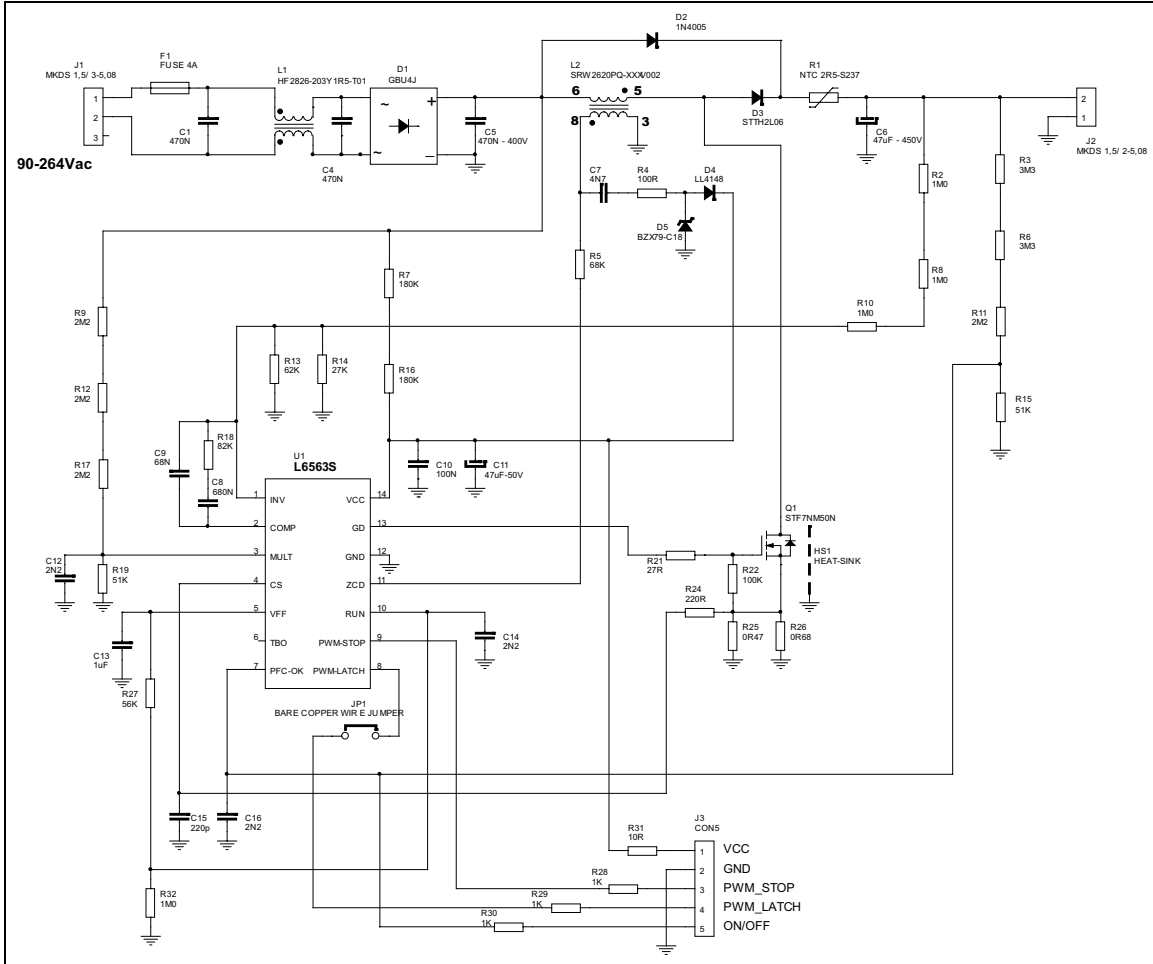
Figure 48. Demonstration board EVL6563S-100W, wide-range mains: electrical schematic
