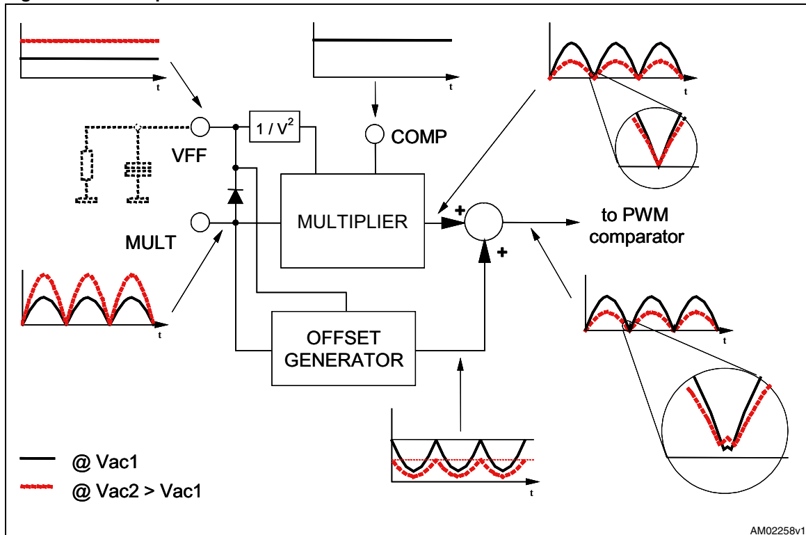
Figure 38. THD optimizer circuit
